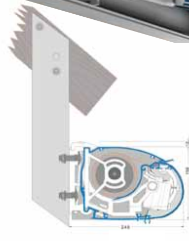
Rafter Fix
