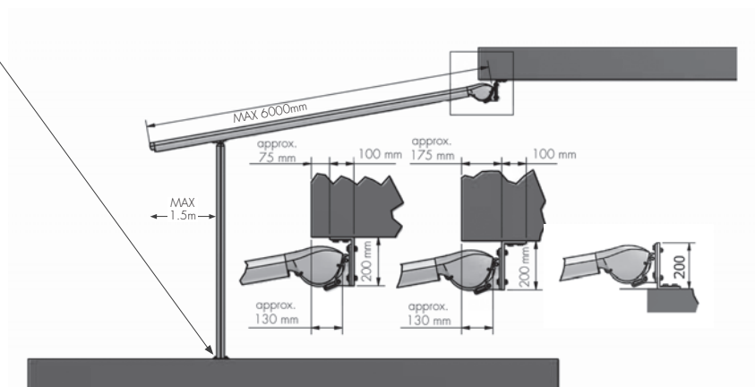
Ceiling installation of VARIO PERGOLA with angle towards the back or towards the front
